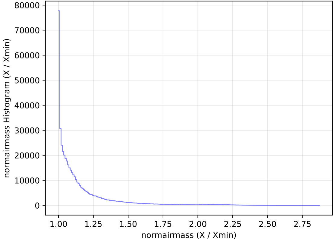
too_elab_heavy_r128_d3_ugrizy_v3.4_10yrs WFD r band: normairmass Histogram
