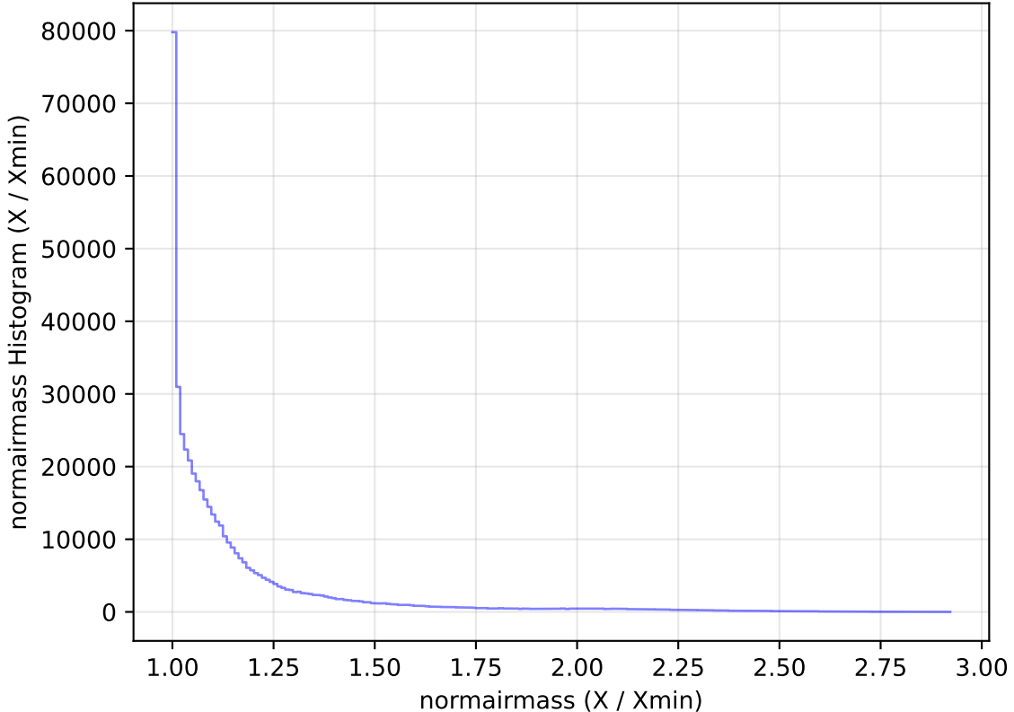
too_elab_heavy_r128_d3_ugrizy_v3.4_10yrs WFD i band: normairmass Histogram
