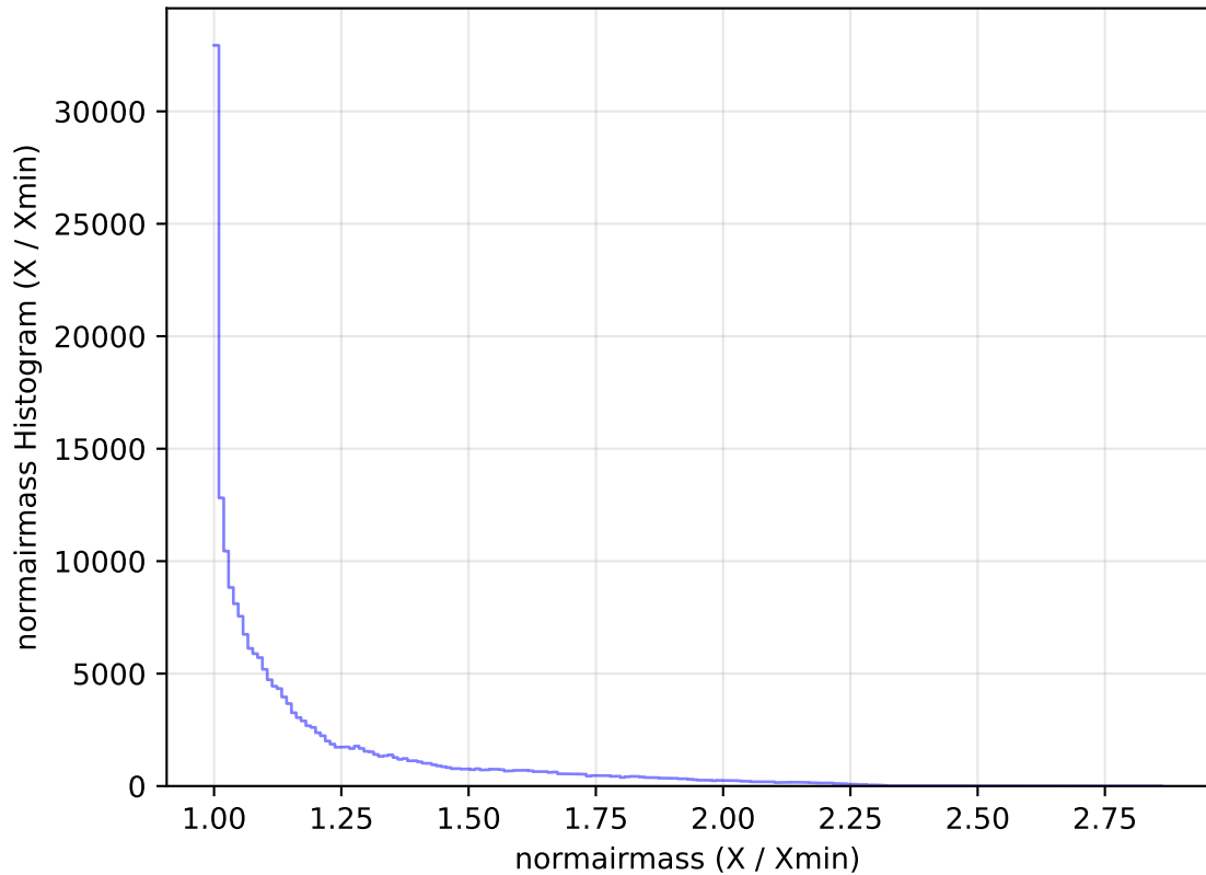
too_elab_heavy_r128_d3_ugrizy_v3.4_10yrs WFD g band: normairmass Histogram
