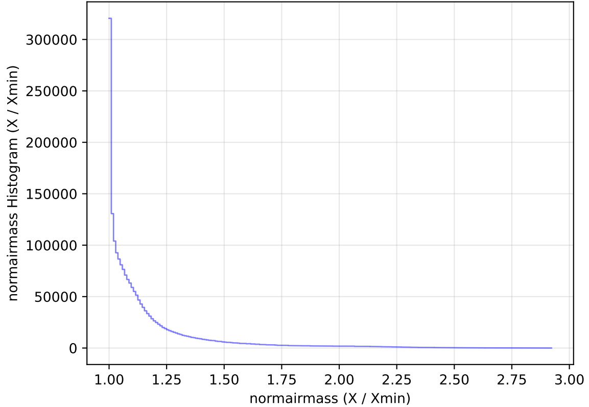
too_elab_heavy_r128_d3_ugrizy_v3.4_10yrs WFD all bands: normairmass Histogram
