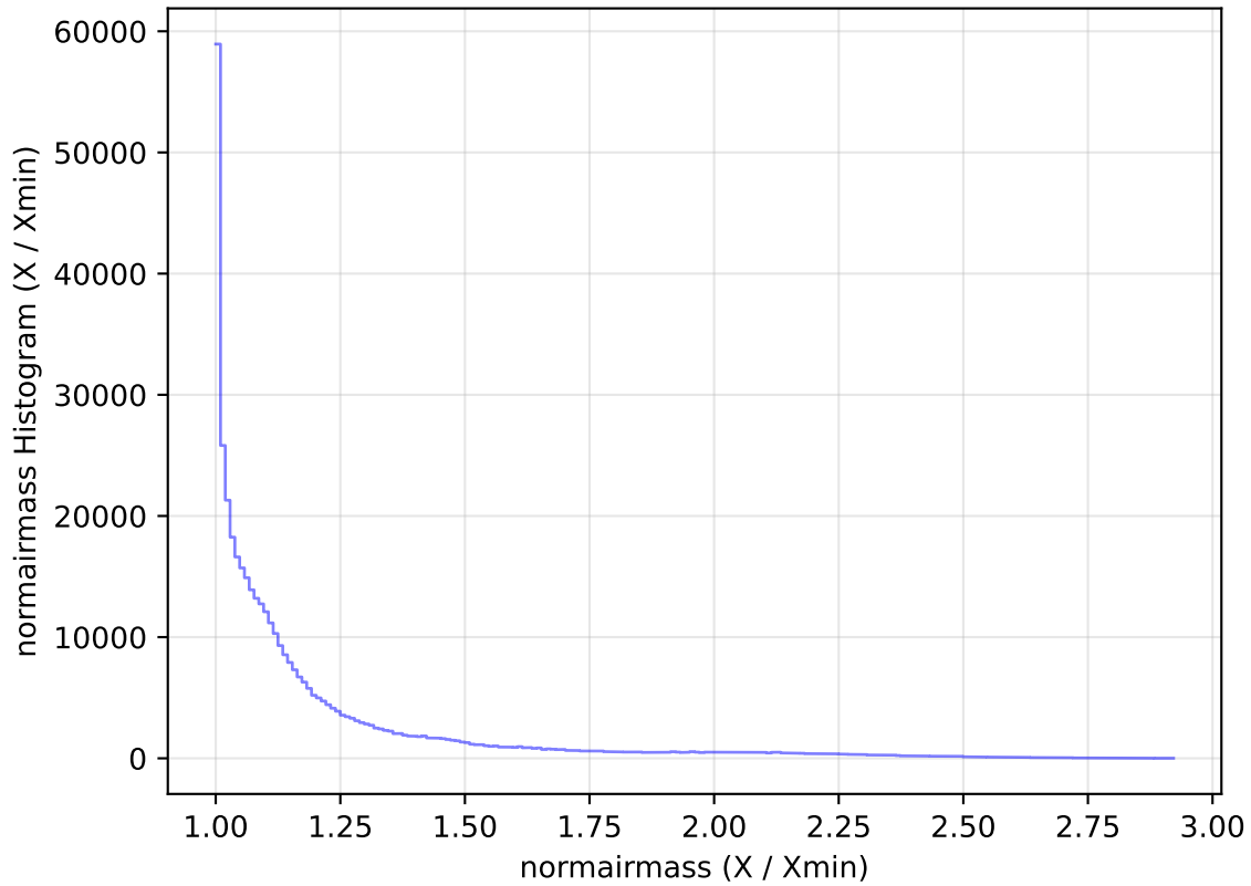
too_elab_heavy_r128_d3_ugrizy_v3.4_10yrs All sky z band: normairmass Histogram
