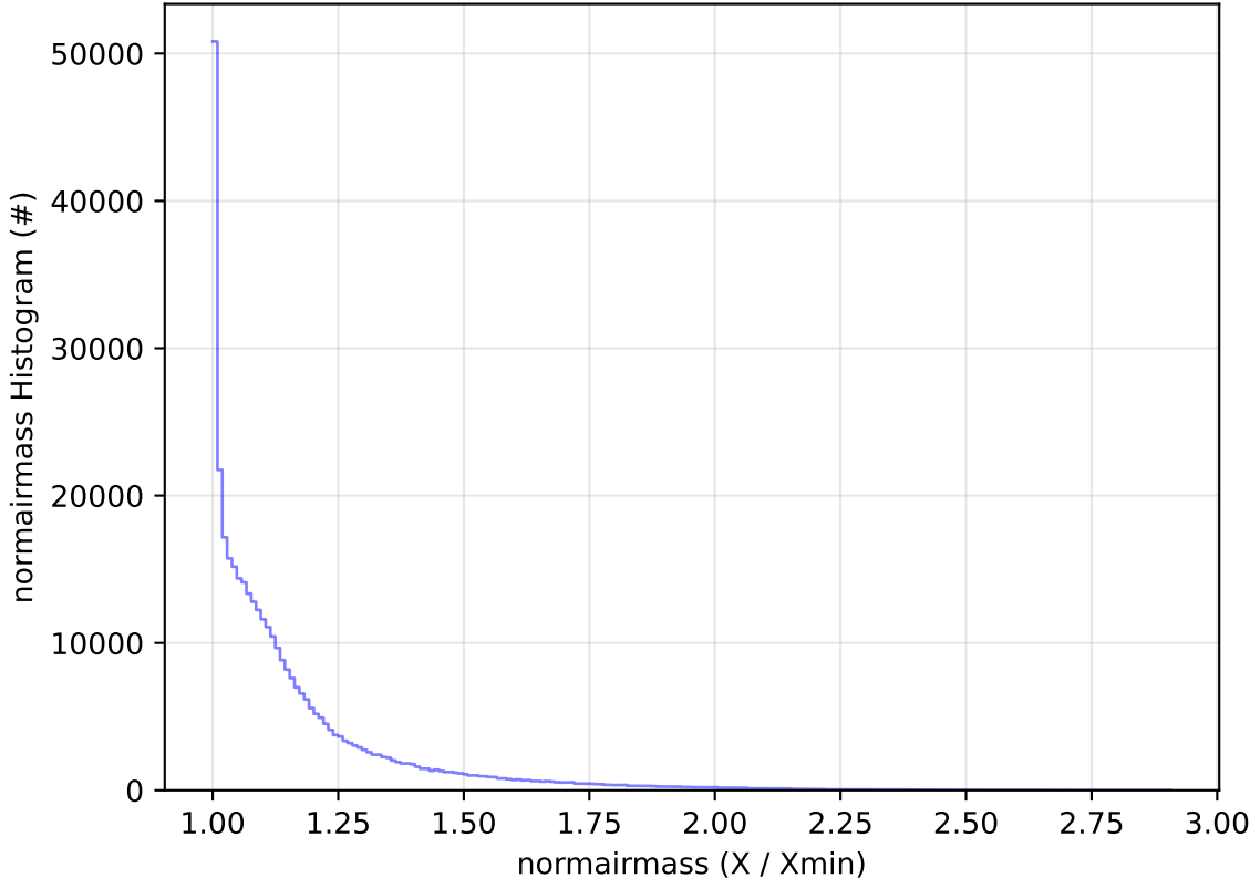
too_elab_heavy_r128_d3_ugrizy_v3.4_10yrs All sky y band: normairmass Histogram
