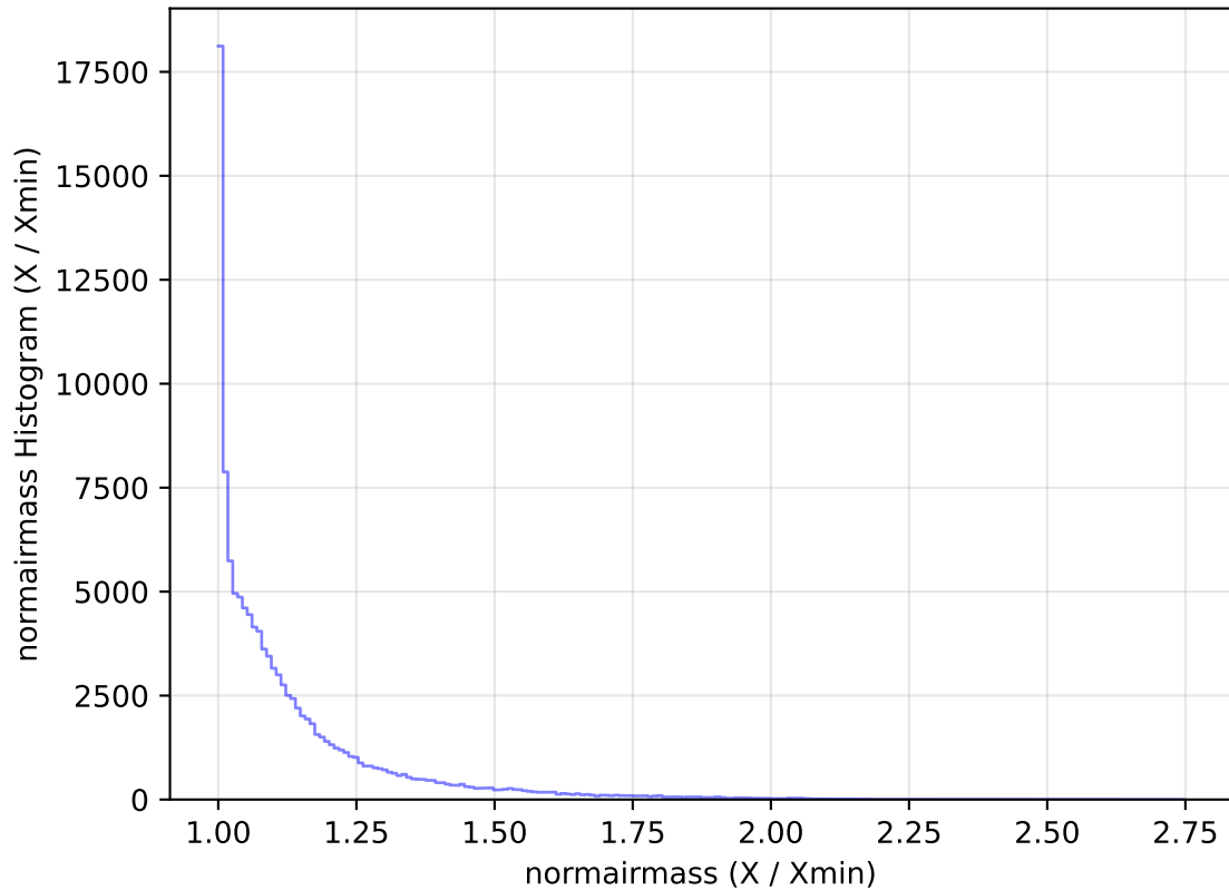
too_elab_heavy_r128_d3_ugrizy_v3.4_10yrs All sky u band: normairmass Histogram
