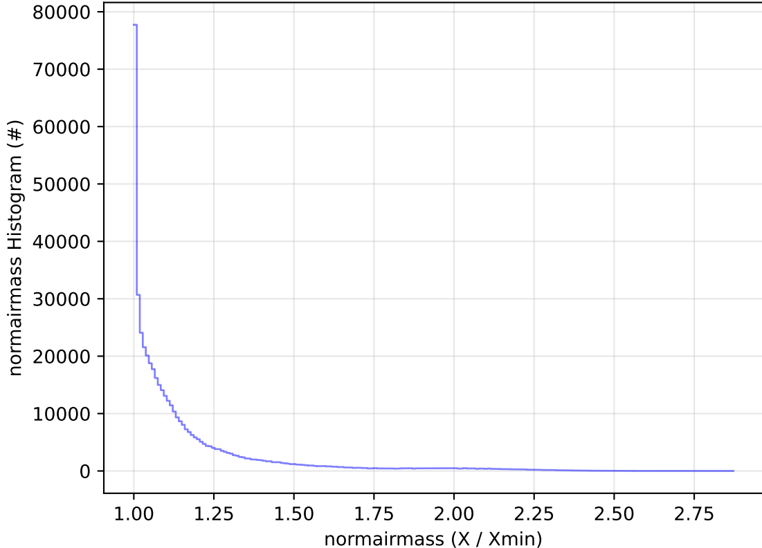
too_elab_heavy_r128_d3_ugrizy_v3.4_10yrs All sky r band: normairmass Histogram
