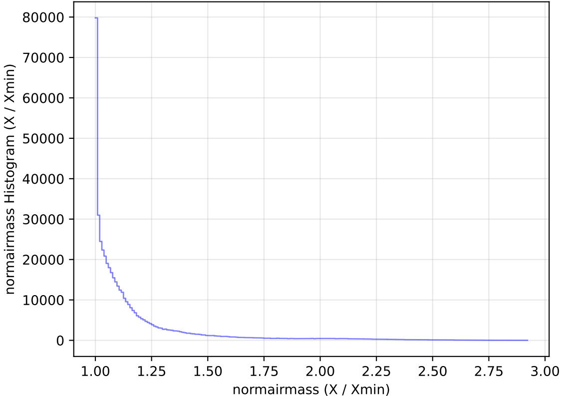
too_elab_heavy_r128_d3_ugrizy_v3.4_10yrs All sky i band: normairmass Histogram
