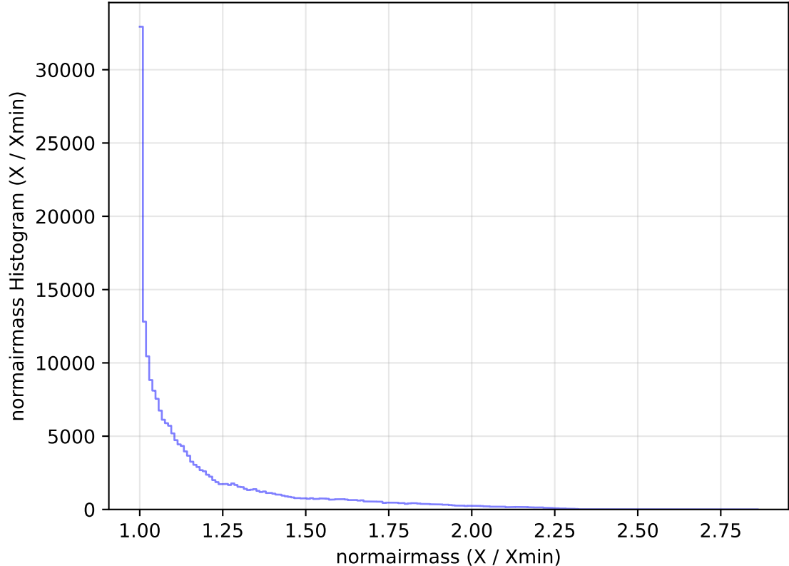
too_elab_heavy_r128_d3_ugrizy_v3.4_10yrs All sky g band: normairmass Histogram
