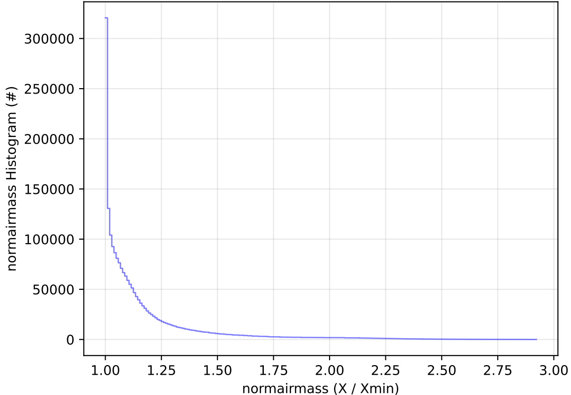
too_elab_heavy_r128_d3_ugrizy_v3.4_10yrs All sky all bands: normairmass Histogram
