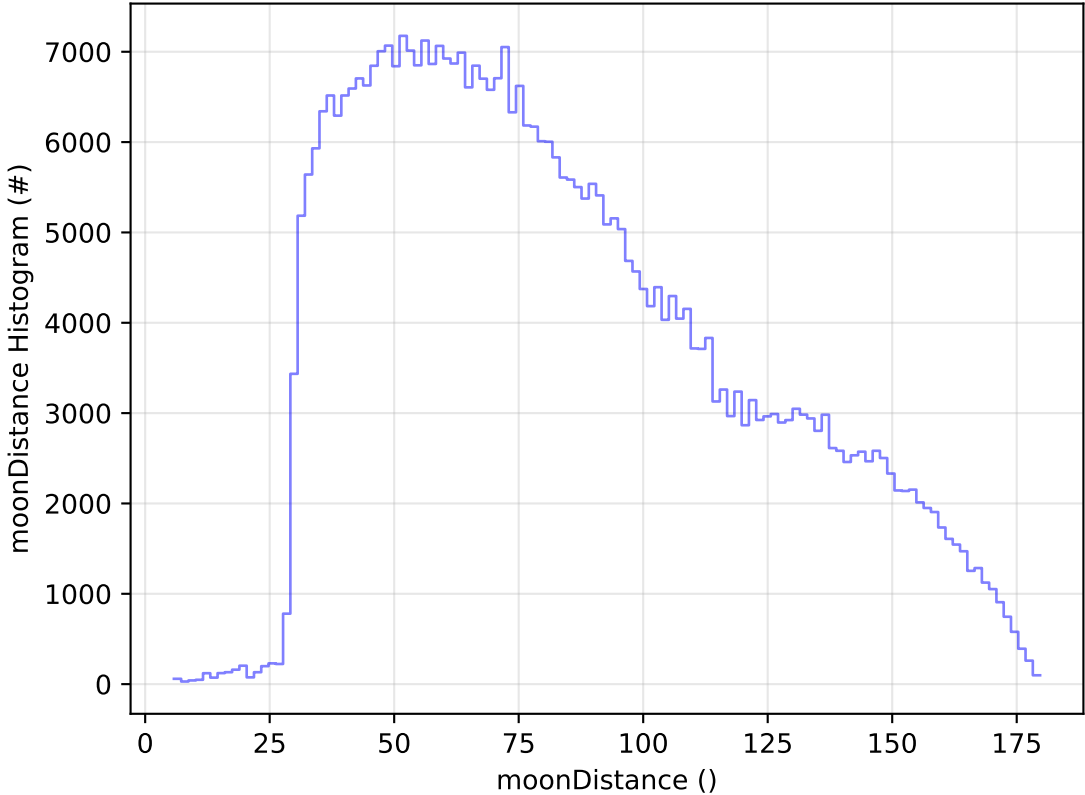
too_elab_heavy_r128_d3_ugrily_v3.4_10yrs WFD z band: moonDistance Histogram
