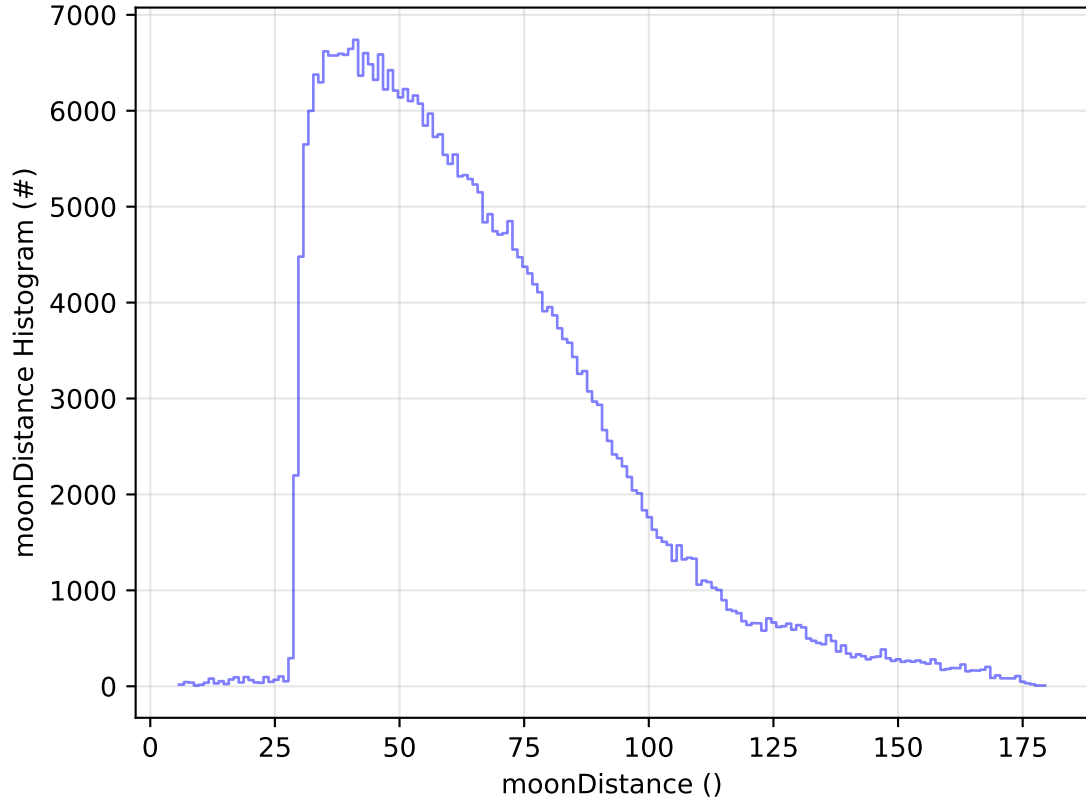
too_elab_heavy_r128_d3_ugrizy_v3.4_10yrs WFD y band: moonDistance Histogram
