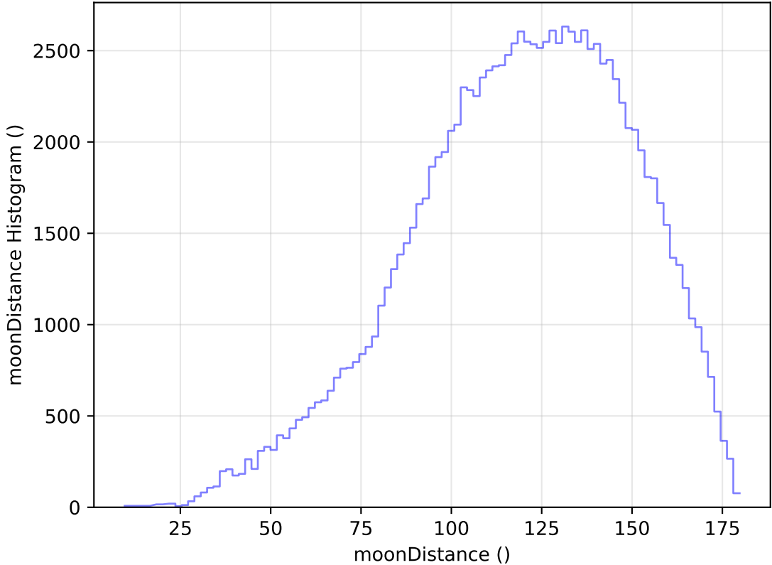
too_elab_heavy_r128_d3_ugrizy_v3.4_10yrs WFD u band: moonDistance Histogram
