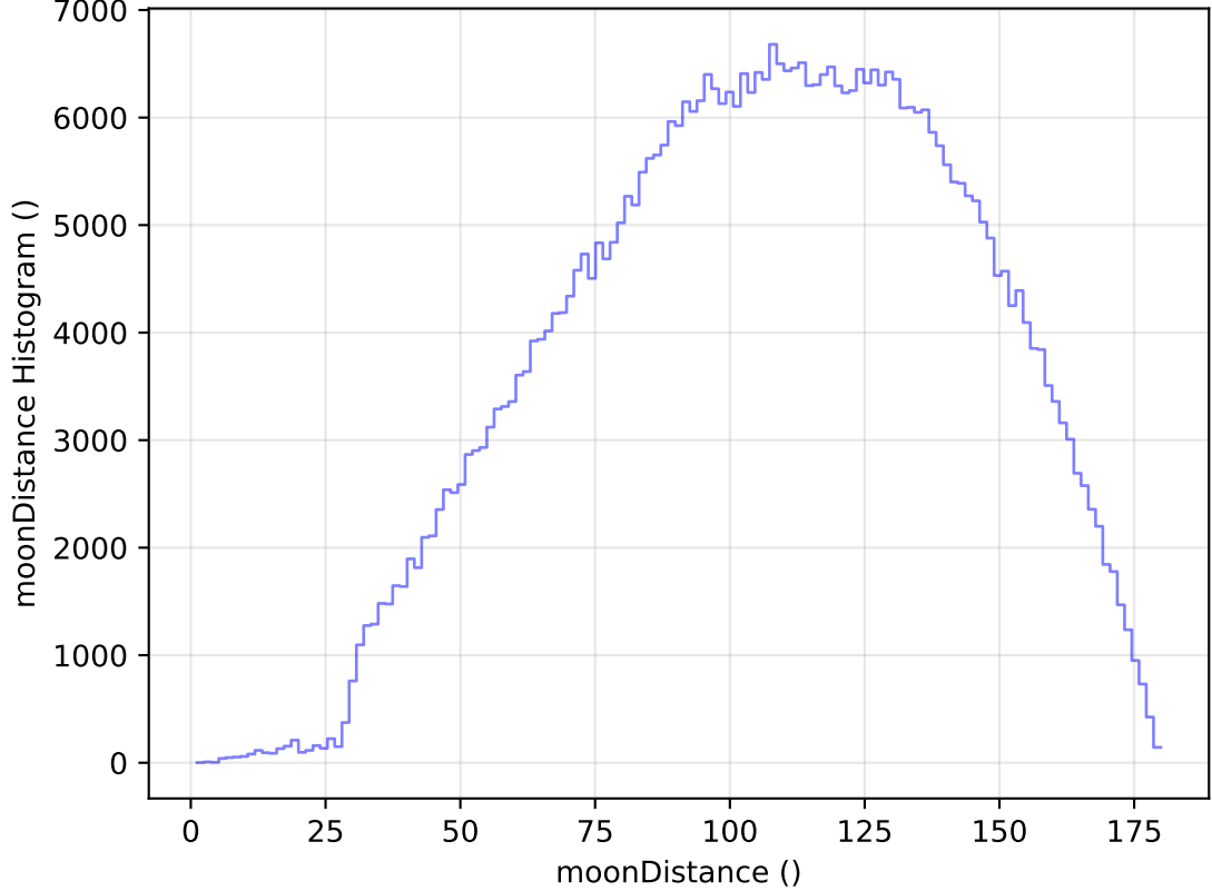
too_elab_heavy_r128_d3_ugrizy_v3.4_10yrs WFD r band: moonDistance Histogram
