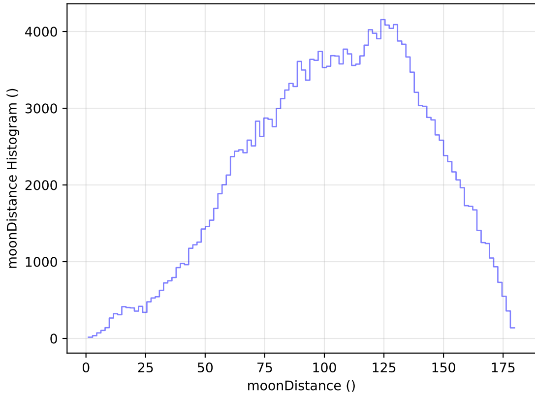
too_elab_heavy_r128_d3_ugrizy_v3.4_10yrs WFD g band: moonDistance Histogram
