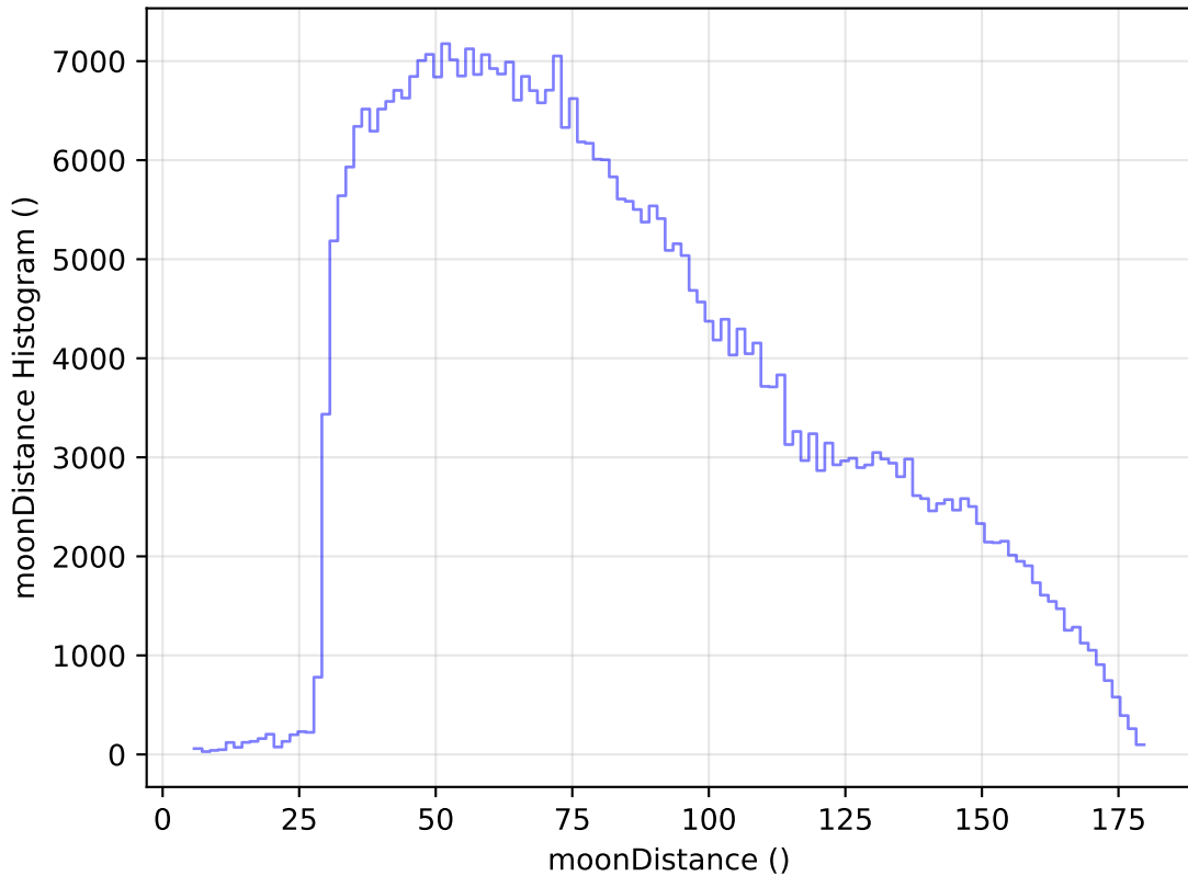
too_elab_heavy_r128_d3_ugrizy_v3.4_10yrs All sky z band: moonDistance Histogram
