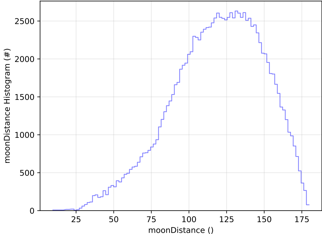
too_elab_heavy_r128_d3_ugrizy_v3.4_10yrs All sky u band: moonDistance Histogram
