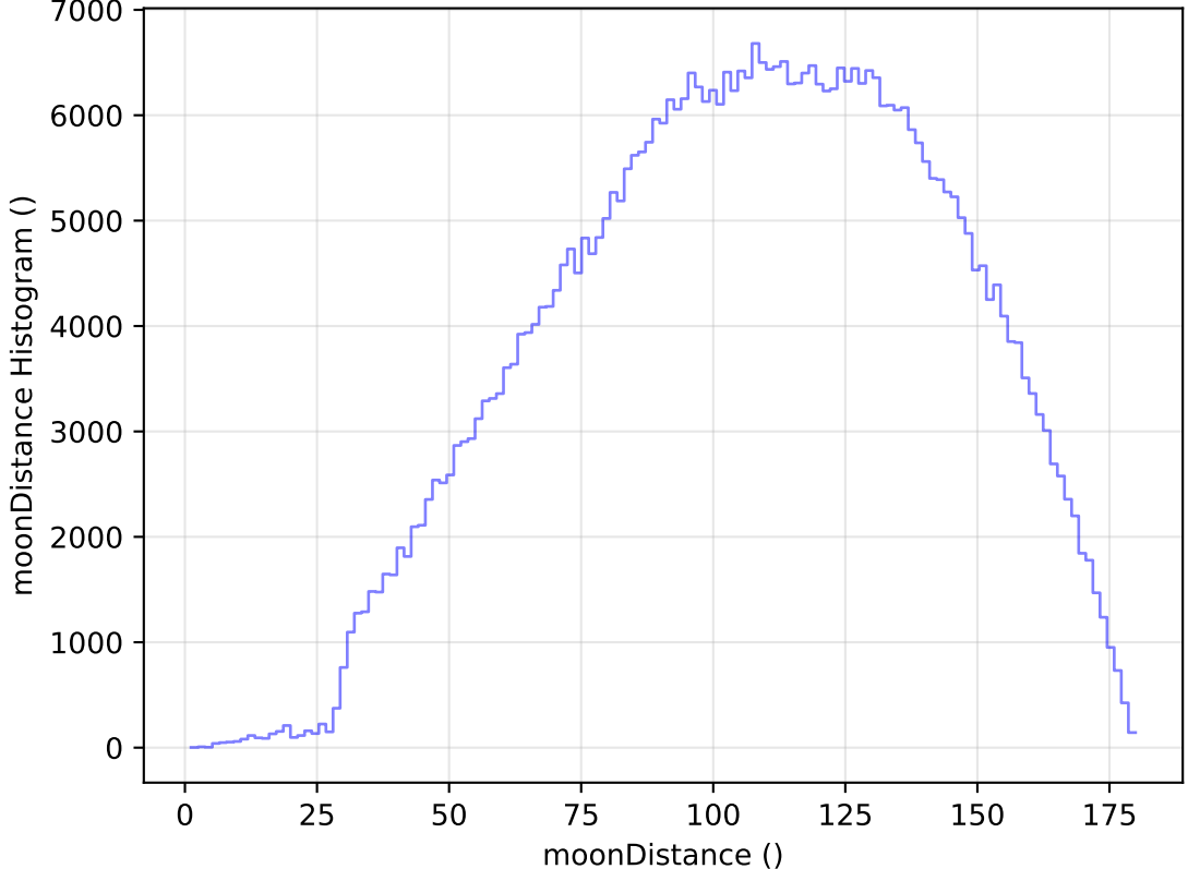
too_elab_heavy_r128_d3_ugrizy_v3.4_10yrs All sky r band: moonDistance Histogram
