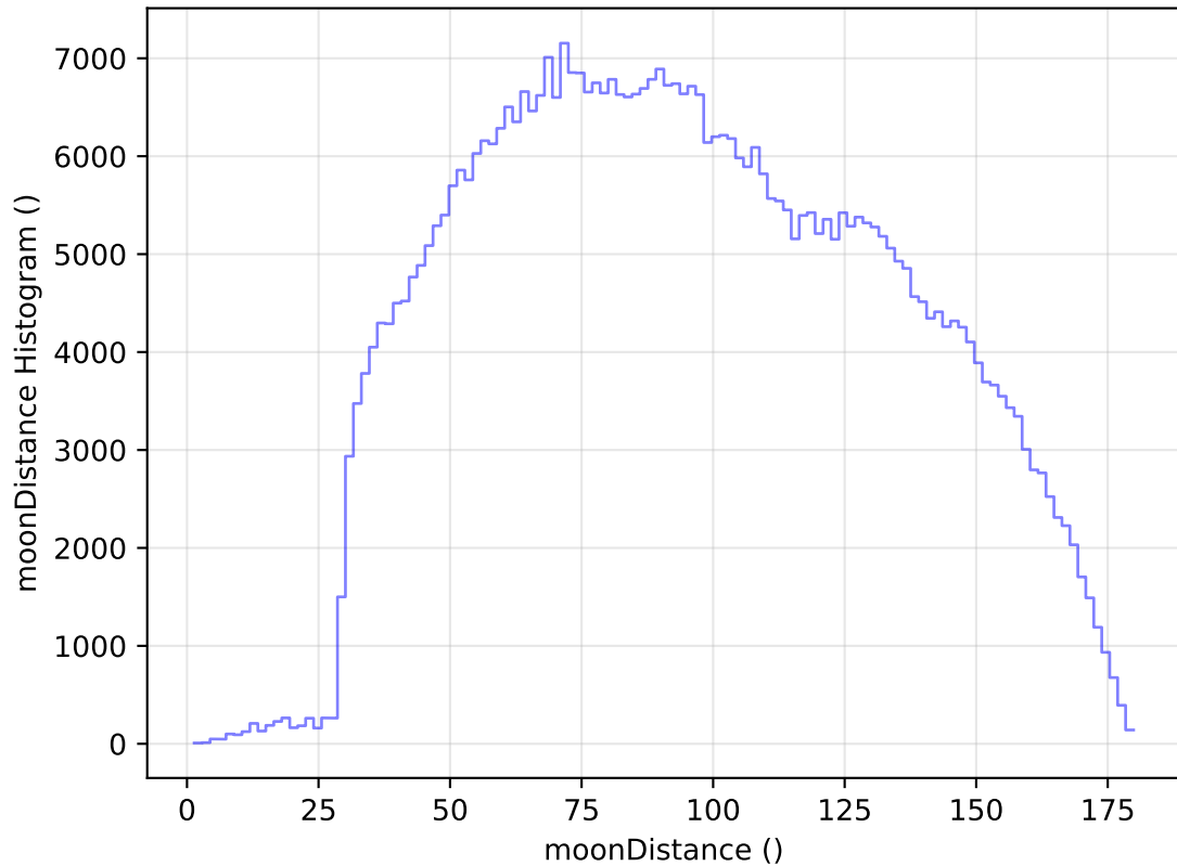
too_elab_heavy_r128_d3_ugrizy_v3.4_10yrs All sky i band: moonDistance Histogram
