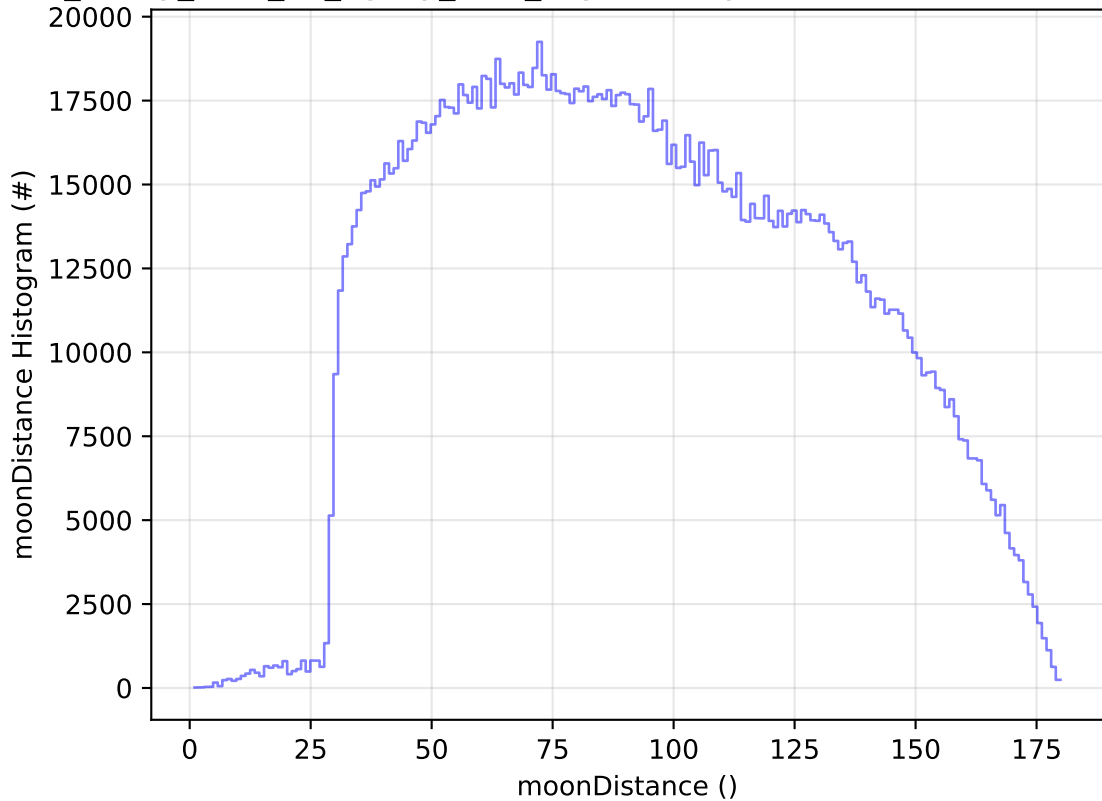
too_elab_heavy_r128_d3_ugrizy_v3.4_10yrs All sky all bands: moonDistance Histogram
