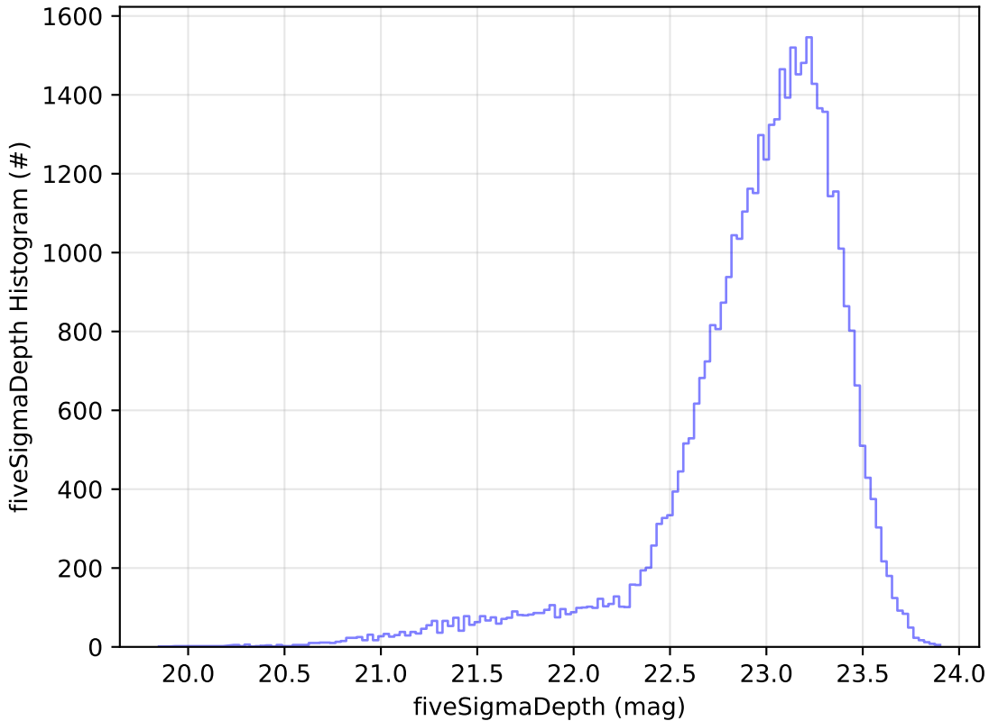
too_elab_heavy_r128_d3_ugrizy_v3.4_10yrs Yr 1 z band: fiveSigmaDepth Histogram
