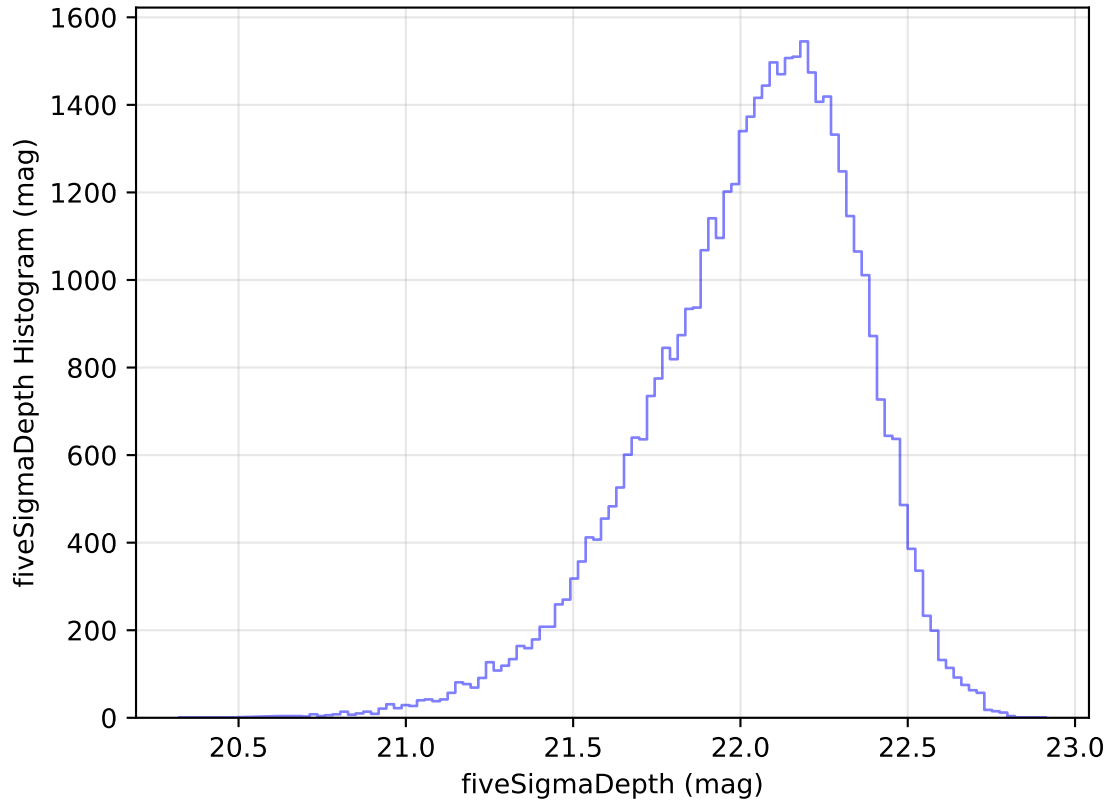
too_elab_heavy_r128_d3_ugrizy_v3.4_10yrs Yr 1 y band: fiveSigmaDepth Histogram
