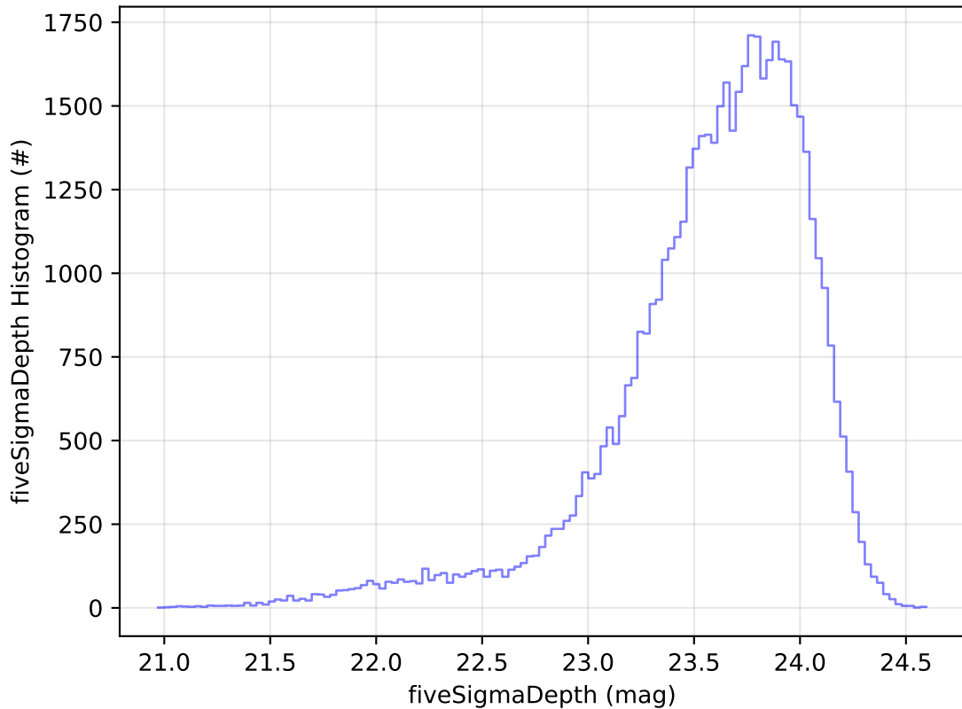
too_elab_heavy_r128_d3_ugrizy_v3.4_10yrs Yr 1 i band: fiveSigmaDepth Histogram
