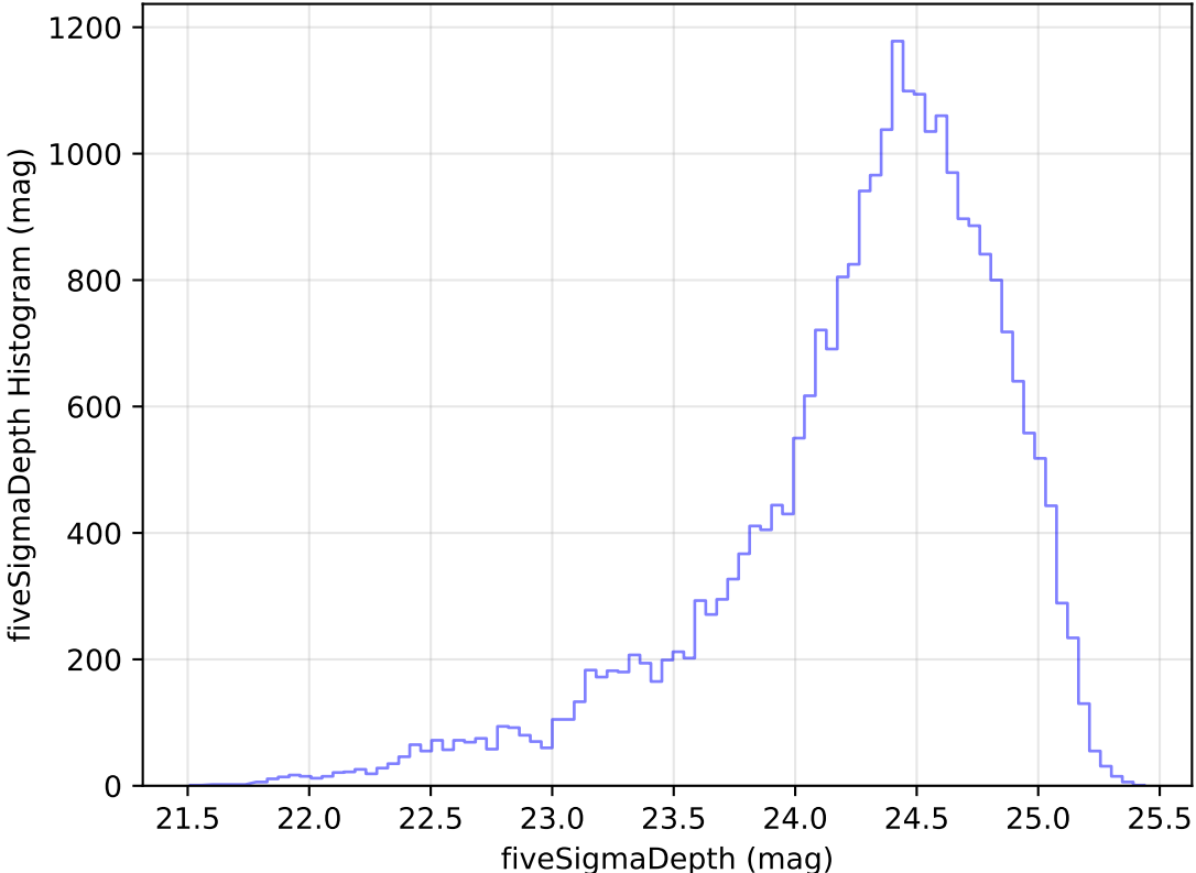
too_elab_heavy_r128_d3_ugrizy_v3.4_10yrs Yr 1 g band: fiveSigmaDepth Histogram
