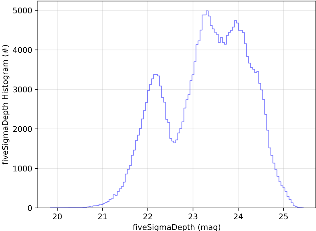
too_elab_heavy_r128_d3_ugrizy_v3.4_10yrs Yr 1 all bands: fiveSigmaDepth Histogram
