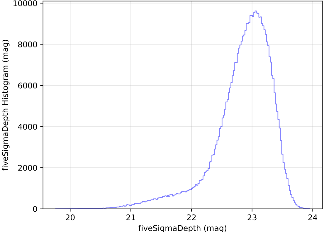
too_elab_heavy_r128_d3_ugrizy_v3.4_10yrs WFD z band: fiveSigmaDepth Histogram
