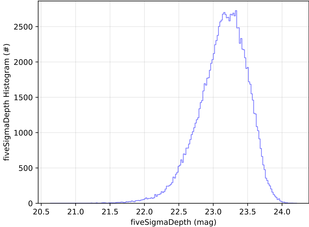
too_elab_heavy_r128_d3_ugrizy_v3.4_10yrs WFD u band: fiveSigmaDepth Histogram
