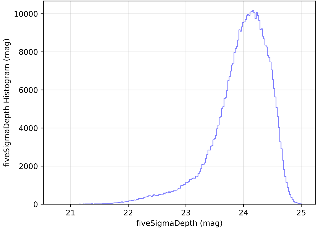
too_elab_heavy_r128_d3_ugrizy_v3.4_10yrs WFD r band: fiveSigmaDepth Histogram
