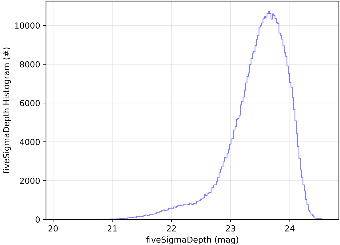
too_elab_heavy_r128_d3_ugrizy_v3.4_10yrs WFD i band: fiveSigmaDepth Histogram
