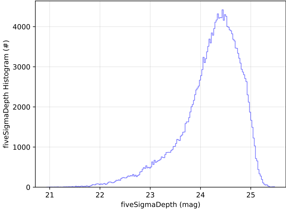
too_elab_heavy_r128_d3_ugrizy_v3.4_10yrs WFD g band: fiveSigmaDepth Histogram
