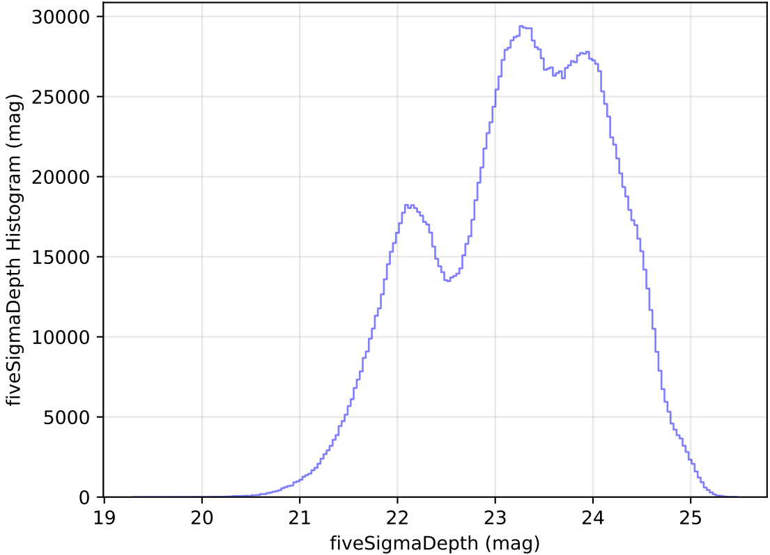
too_elab_heavy_r128_d3_ugrizy_v3.4_10yrs WFD all bands: fiveSigmaDepth Histogram
