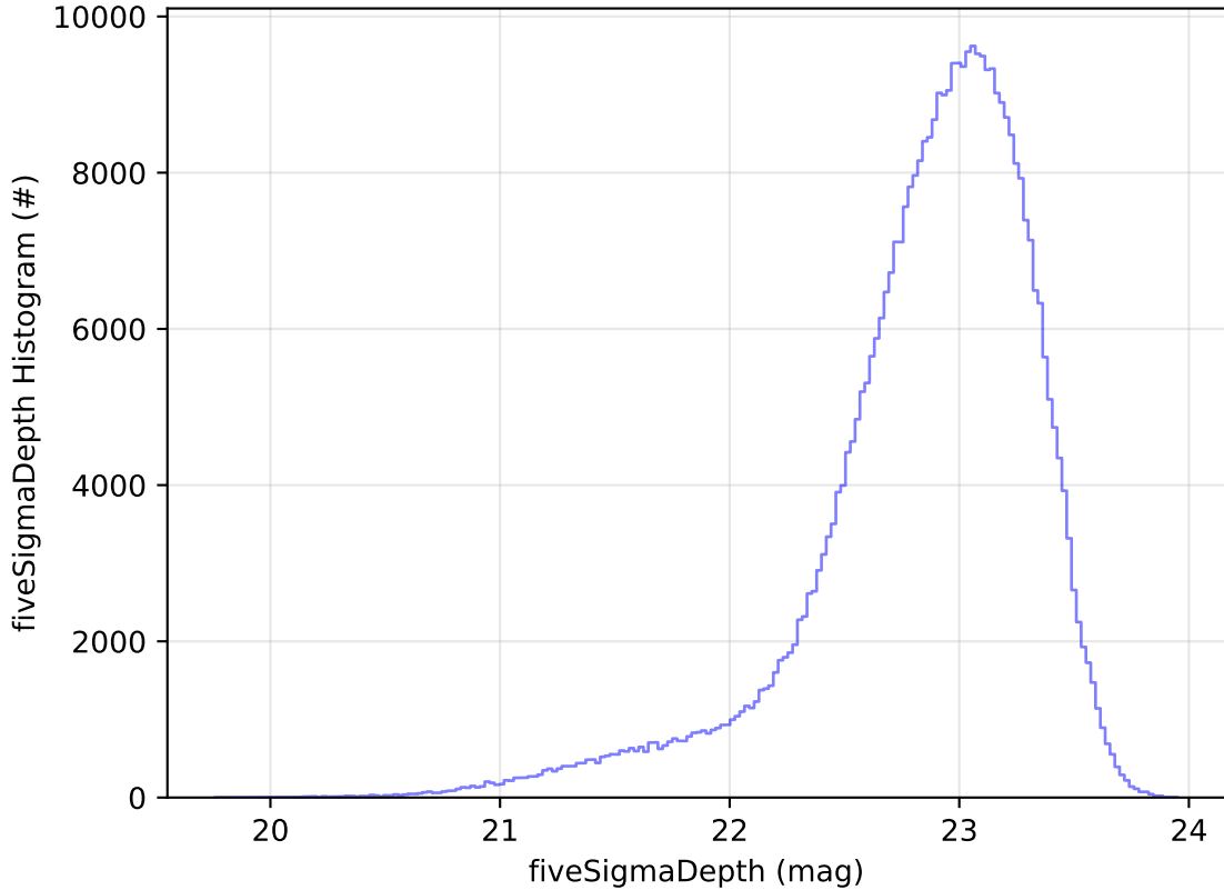
too_elab_heavy_r128_d3_ugrizy_v3.4_10yrs All sky z band: fiveSigmaDepth Histogram
