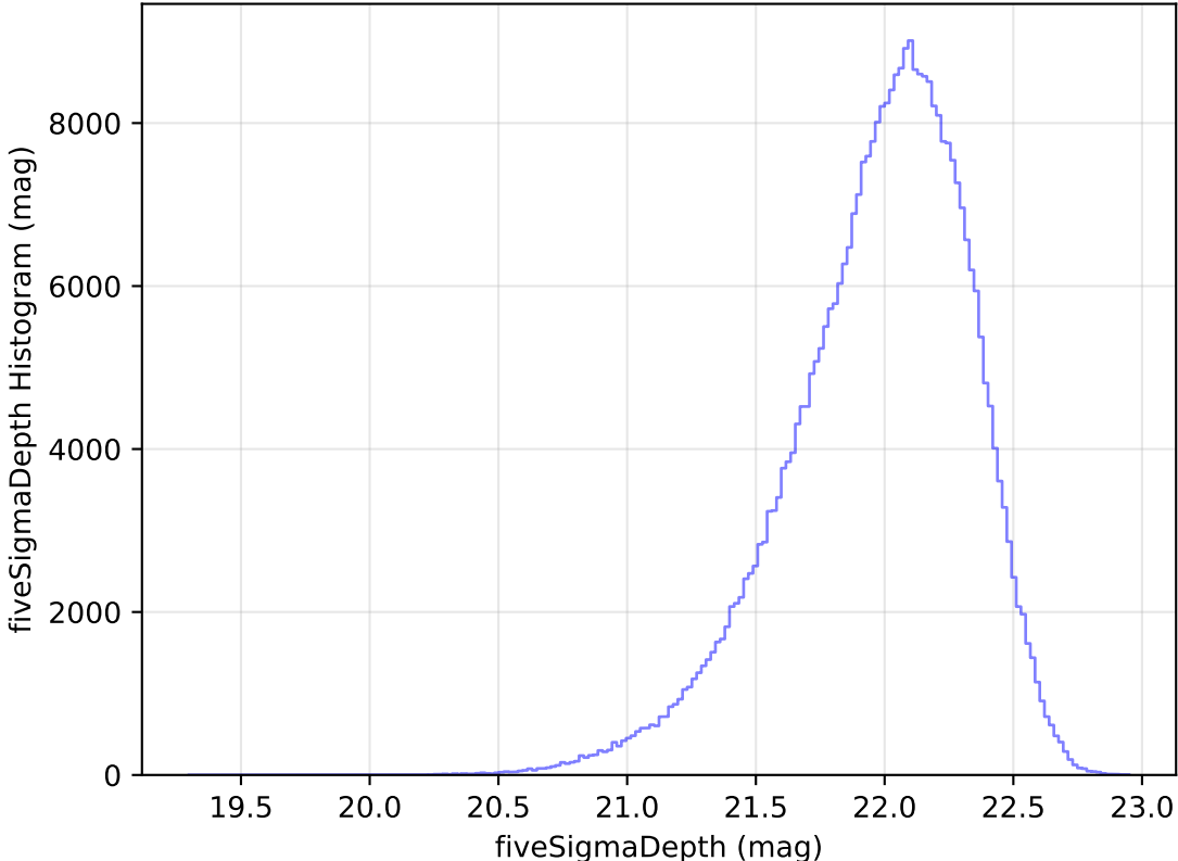
too_elab_heavy_r128_d3_ugrizy_v3.4_10yrs All sky y band: fiveSigmaDepth Histogram
