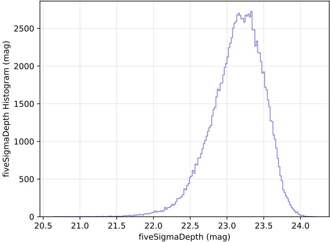
too_elab_heavy_r128_d3_ugrizy_v3.4_10yrs All sky u band: fiveSigmaDepth Histogram
