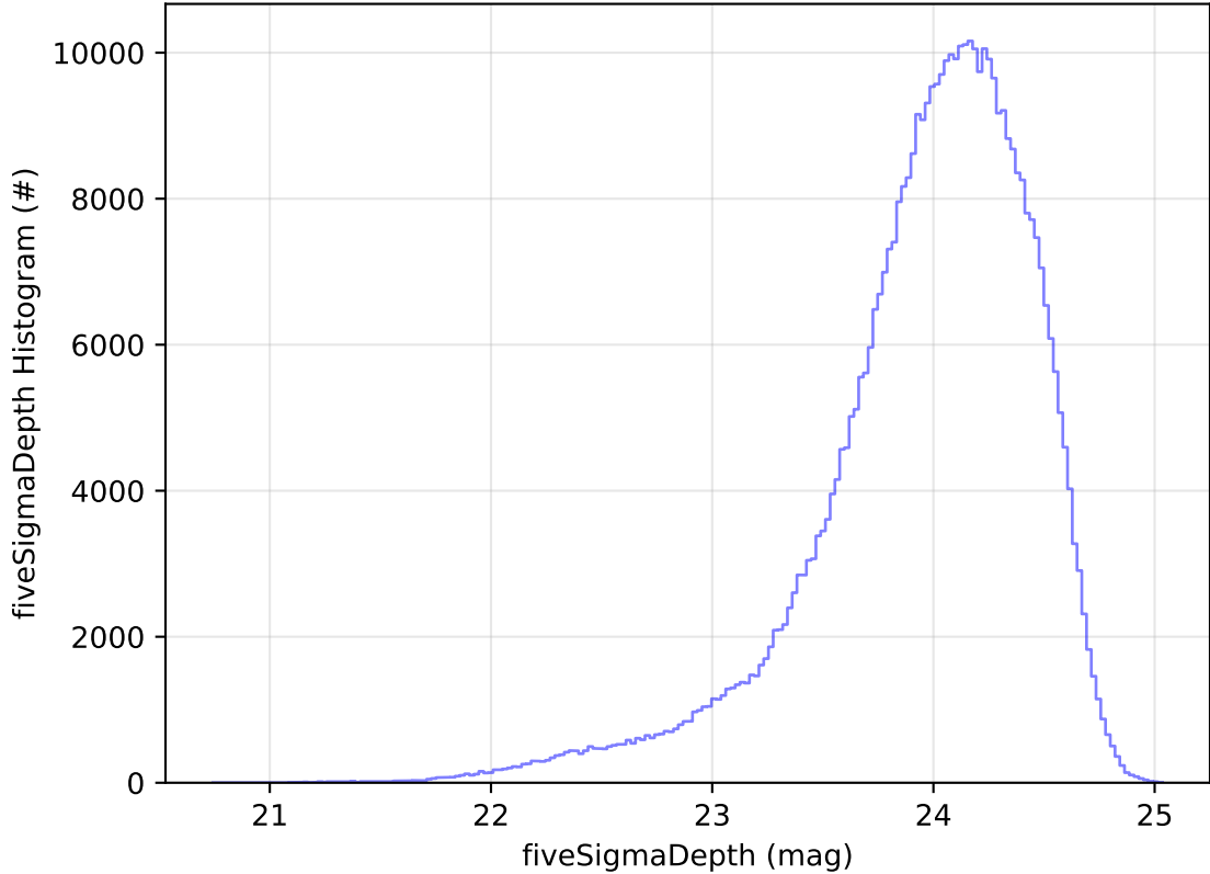
too_elab_heavy_r128_d3_ugrizy_v3.4_10yrs All sky r band: fiveSigmaDepth Histogram
