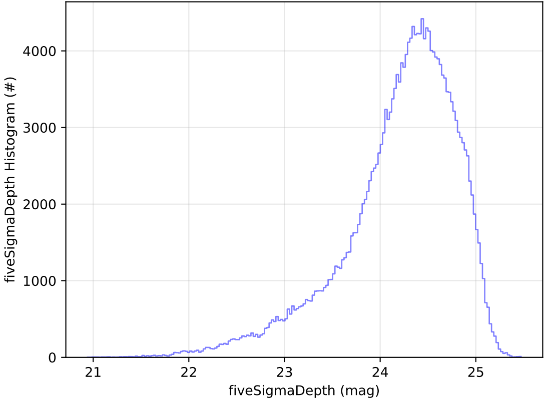
too_elab_heavy_r128_d3_ugrizy_v3.4_10yrs All sky g band: fiveSigmaDepth Histogram
