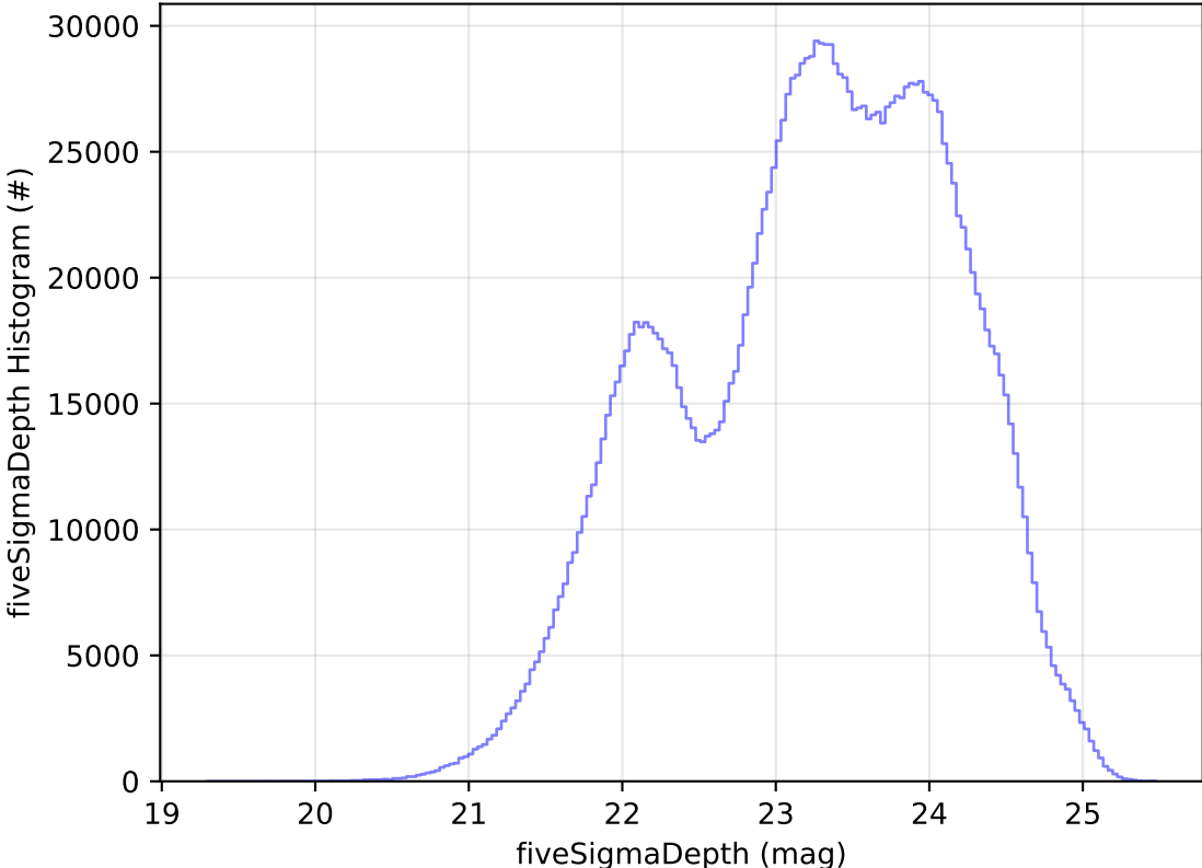
too_elab_heavy_r128_d3_ugrizy_v3.4_10yrs All sky all bands: fiveSigmaDepth Histogram
