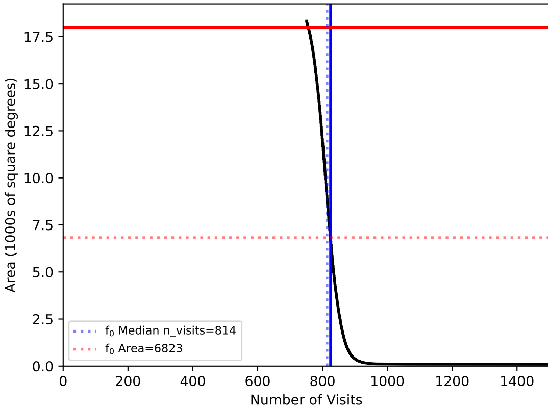
too_elab_heavy_r128_d3_ugrizy_v3.4_10yrs WFD: f0
