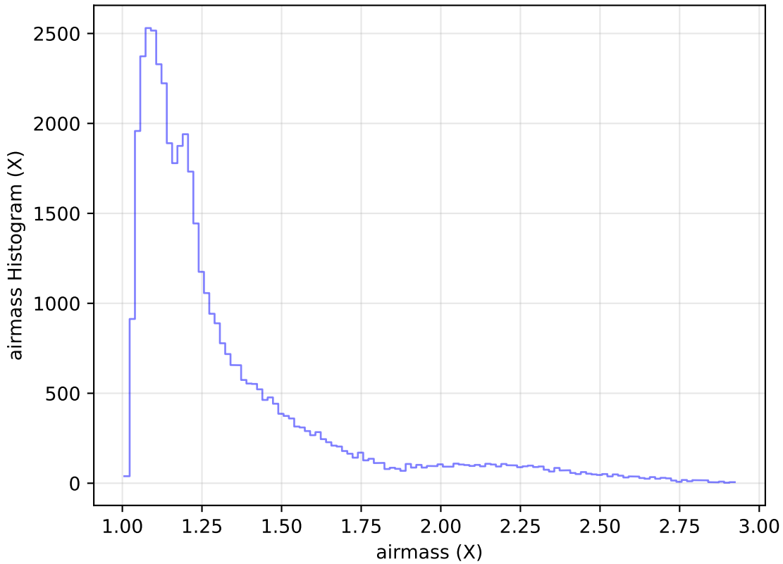
too_elab_heavy_r128_d3_ugrizy_v3.4_10yrs Yr 1 z band: airmass Histogram
