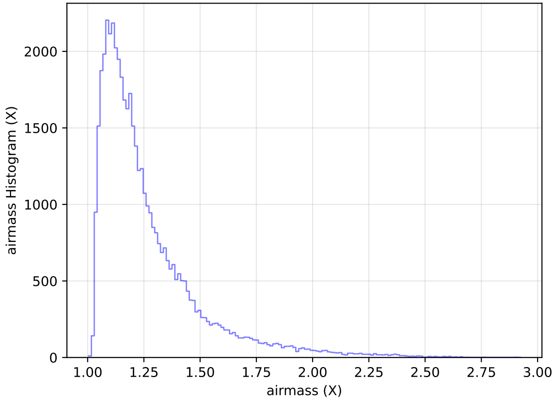
too_elab_heavy_r128_d3_ugrizy_v3.4_10yrs Yr 1 y band: airmass Histogram
