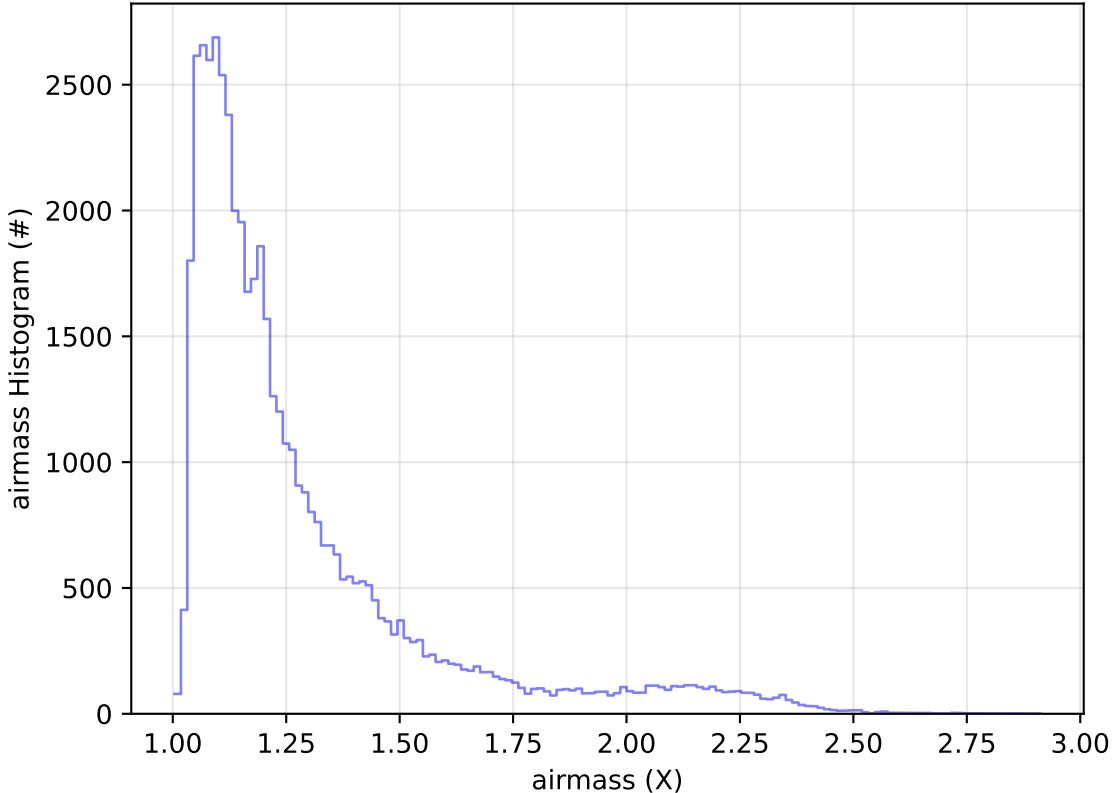
too_elab_heavy_r128_d3_ugrizy_v3.4_10yrs Yr 1 r band: airmass Histogram
