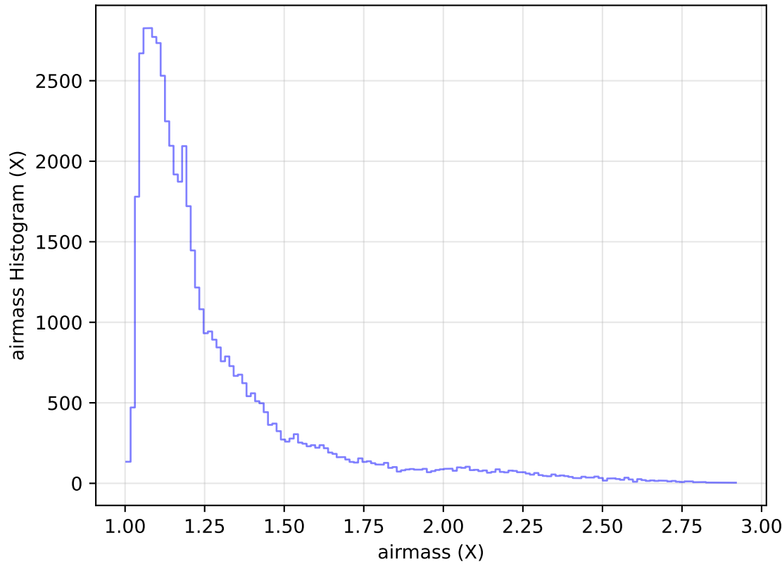
too_elab_heavy_r128_d3_ugrizy_v3.4_10yrs Yr 1 i band: airmass Histogram
