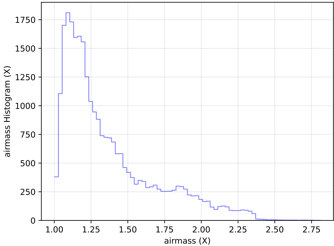
too_elab_heavy_r128_d3_ugrizy_v3.4_10yrs Yr 1 g band: airmass Histogram
