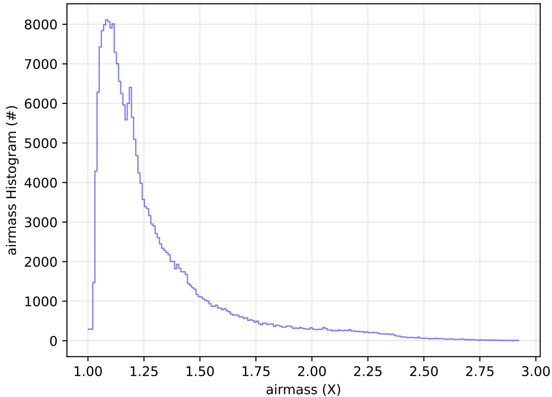
too_elab_heavy_r128_d3_ugrizy_v3.4_10yrs Yr 1 all bands: airmass Histogram
