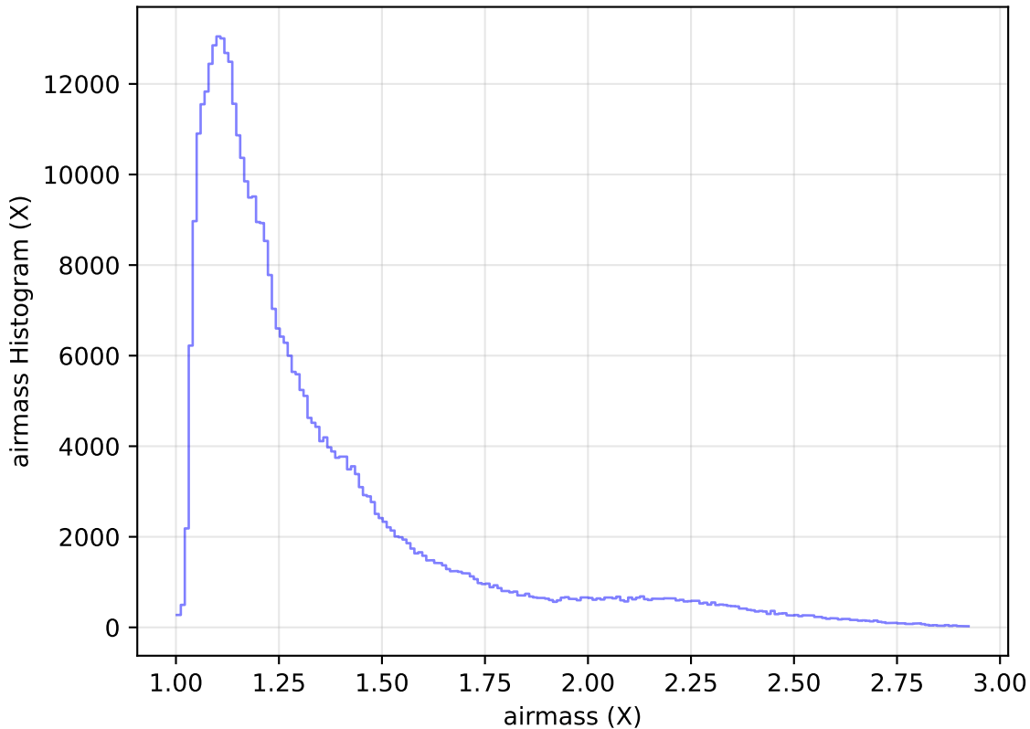
too_elab_heavy_r128_d3_ugrizy_v3.4_10yrs WFD z band: airmass Histogram
