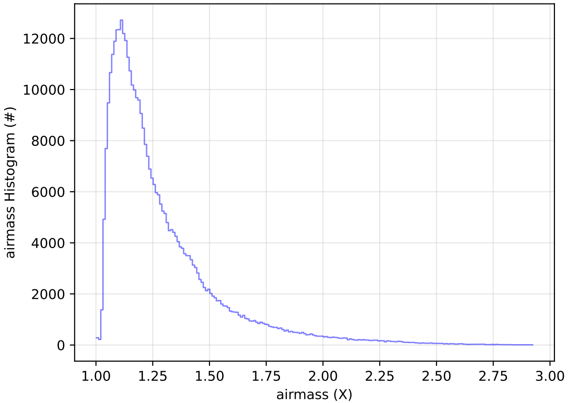
too_elab_heavy_r128_d3_ugrizy_v3.4_10yrs WFD y band: airmass Histogram
