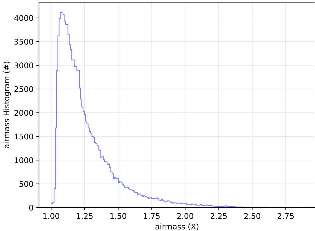
too_elab_heavy_r128_d3_ugrizy_v3.4_10yrs WFD u band: airmass Histogram
