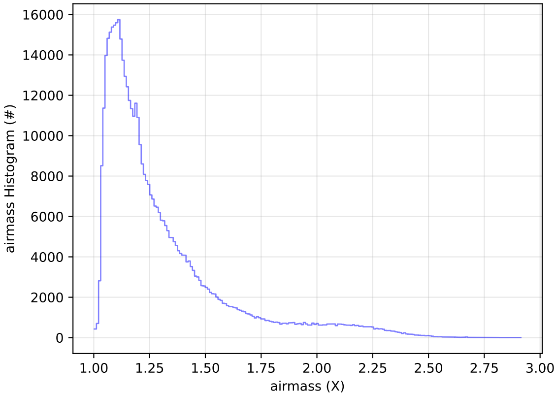
too_elab_heavy_r128_d3_ugrizy_v3.4_10yrs WFD r band: airmass Histogram
