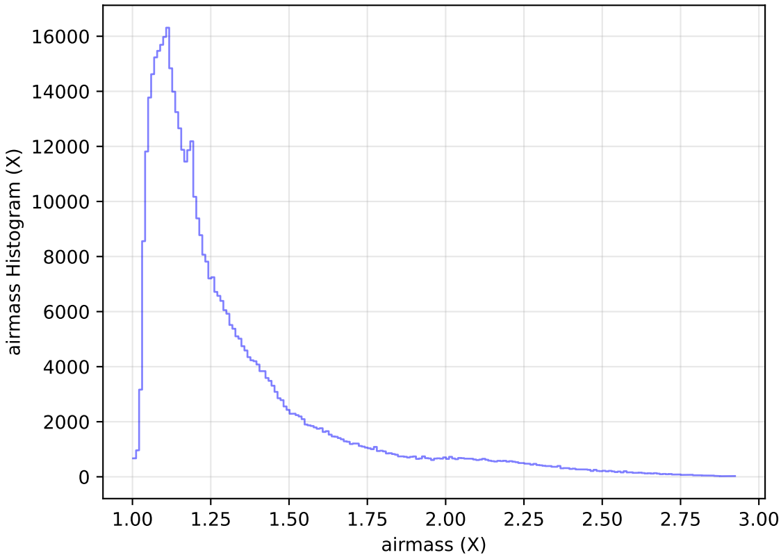
too_elab_heavy_r128_d3_ugrizy_v3.4_10yrs WFD i band: airmass Histogram
